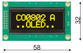
CO-0802A (8Chr. X 2 Lines)
