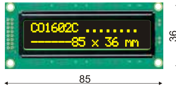
CO-1602C (16Chr. x 2 Lines)
