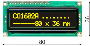
CO-1602A (16Chr. x 2 Lines)
